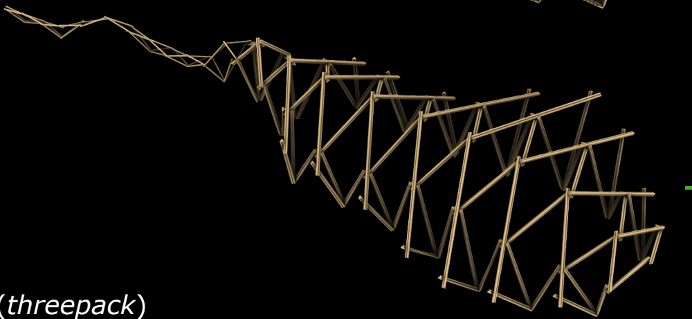
Secondary structure ( hyperbolic paraboloid )
